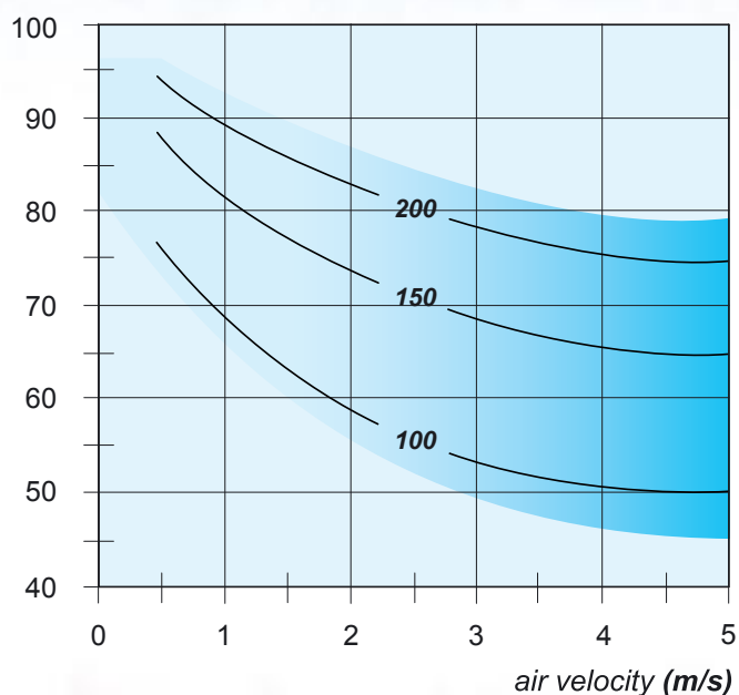
Saturation efficiency (%)
